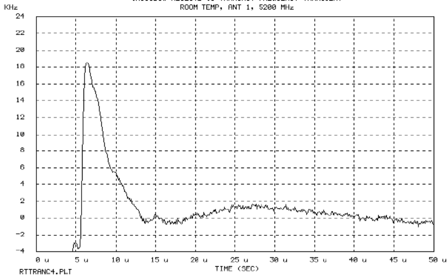
Figure 13-VCO frequency transient
