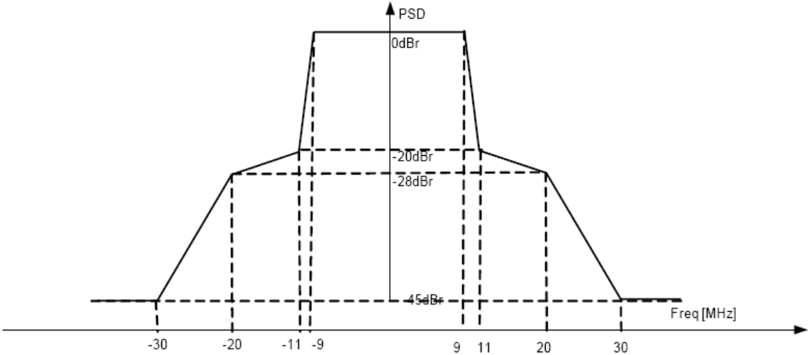
Figure 6-20MHz spectrum mask
