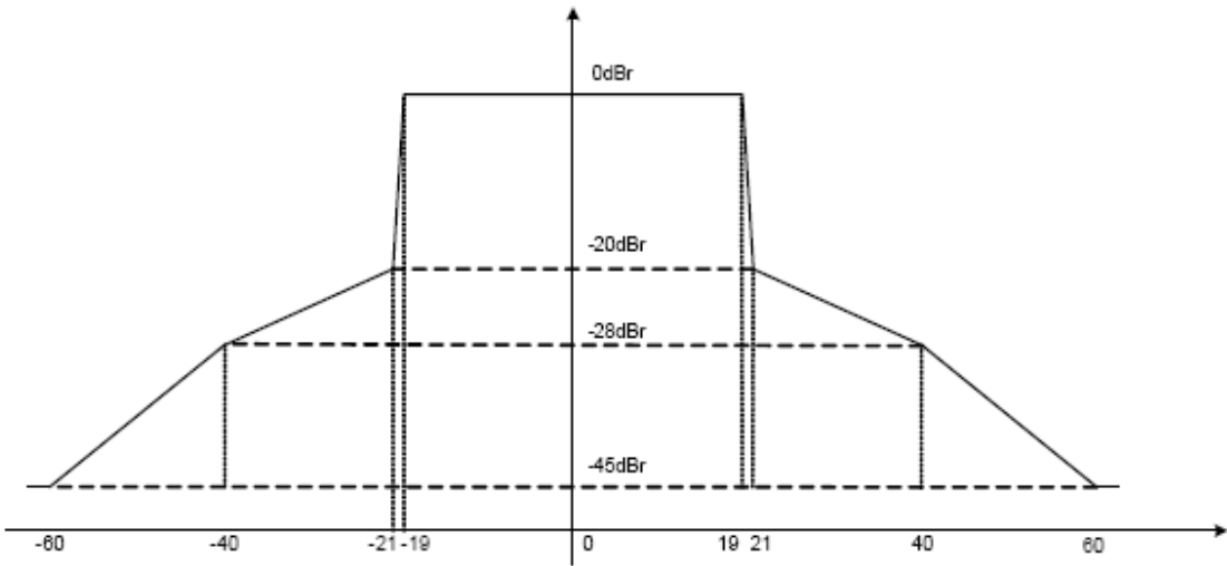
Figure 7-40MHz spectrum mask
