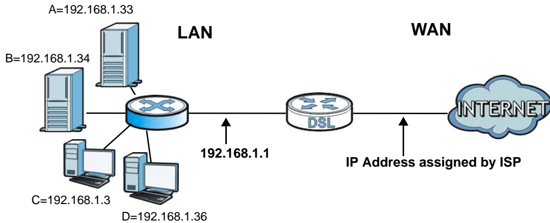
Figure 71 Multiple Servers Behind NAT Example
