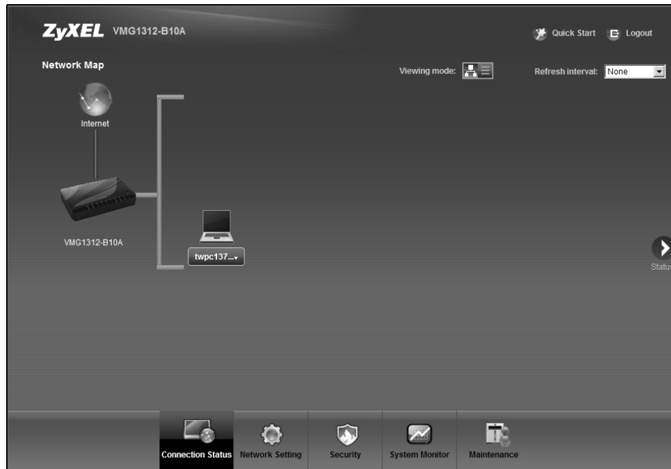
Figure 8 Network Map
