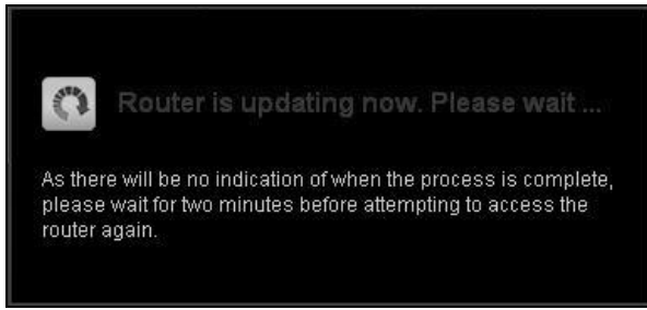
Figure 135 Firmware Uploading
