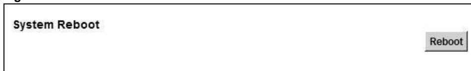
Figure 143 Maintenance > Reboot
