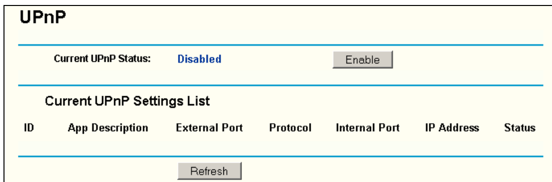
Figure 5-30 UPnP Settings
