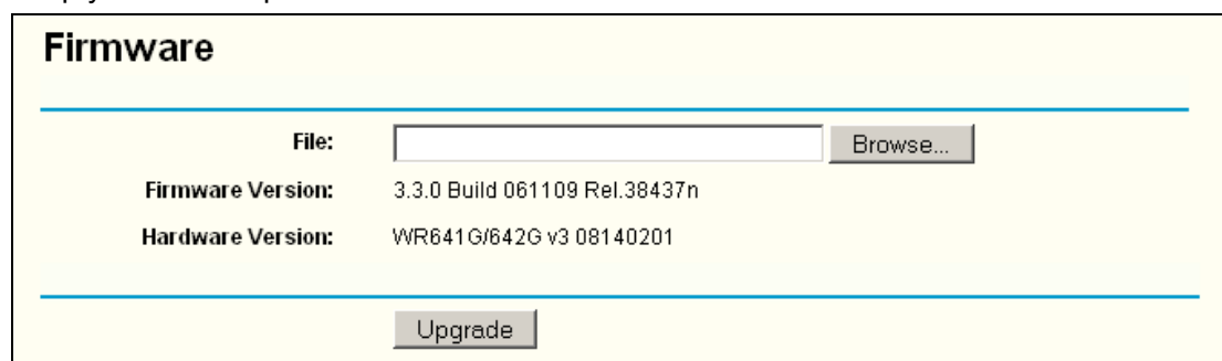
Figure 5-49 Firmware Upgrade
