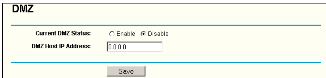
Figure 5-29 DMZ
