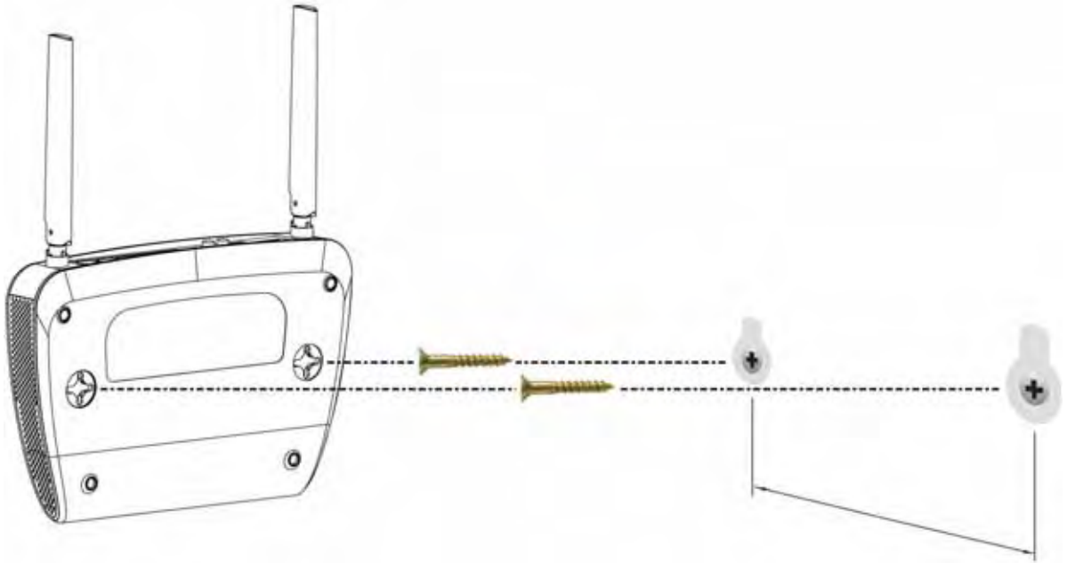
Figure 2 Wall Mounting Example
