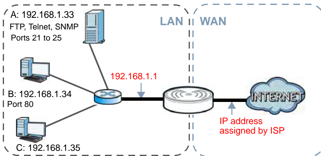
Figure 75 NAT Example
