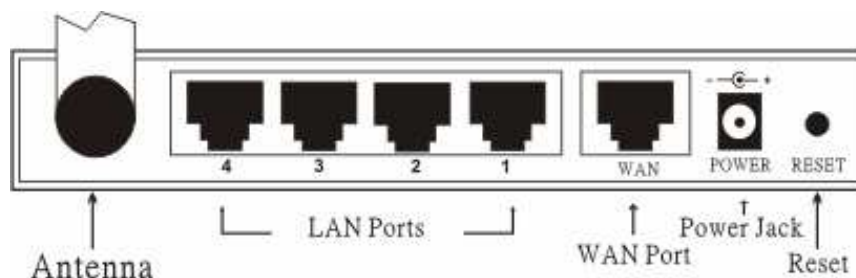
Figure 2. Rear Panel
