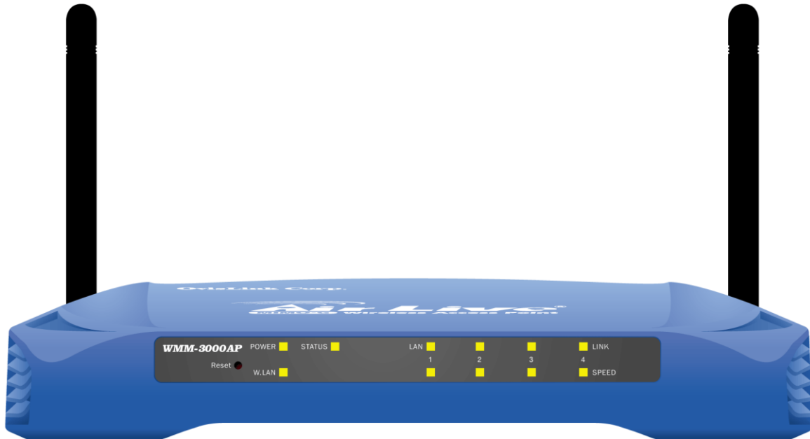
Figure 2-1 Front Panel
