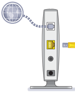
Figure 7. Cable connections
