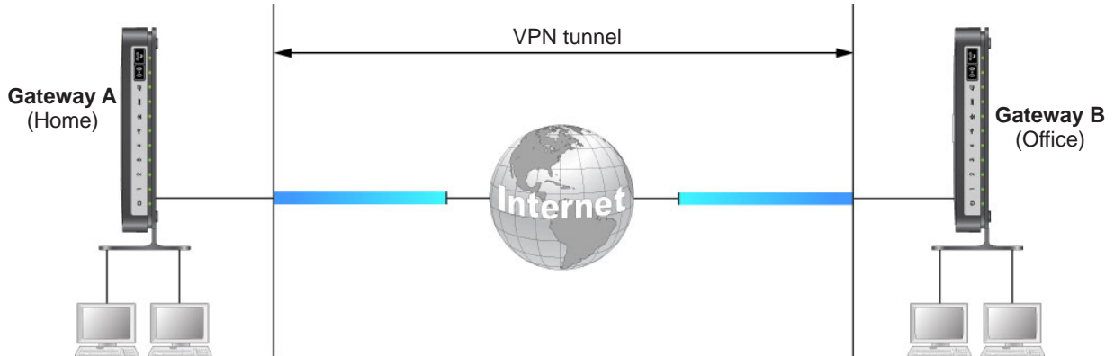
Figure 14. VPN tunnel between networks
