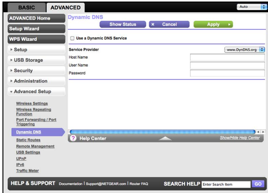
Figure 9. Forward traffic to a changing IP address
