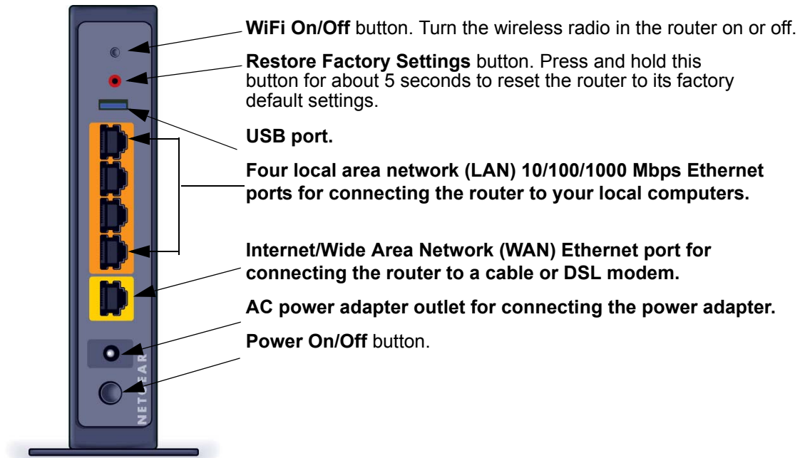
Figure 3. Back panel
