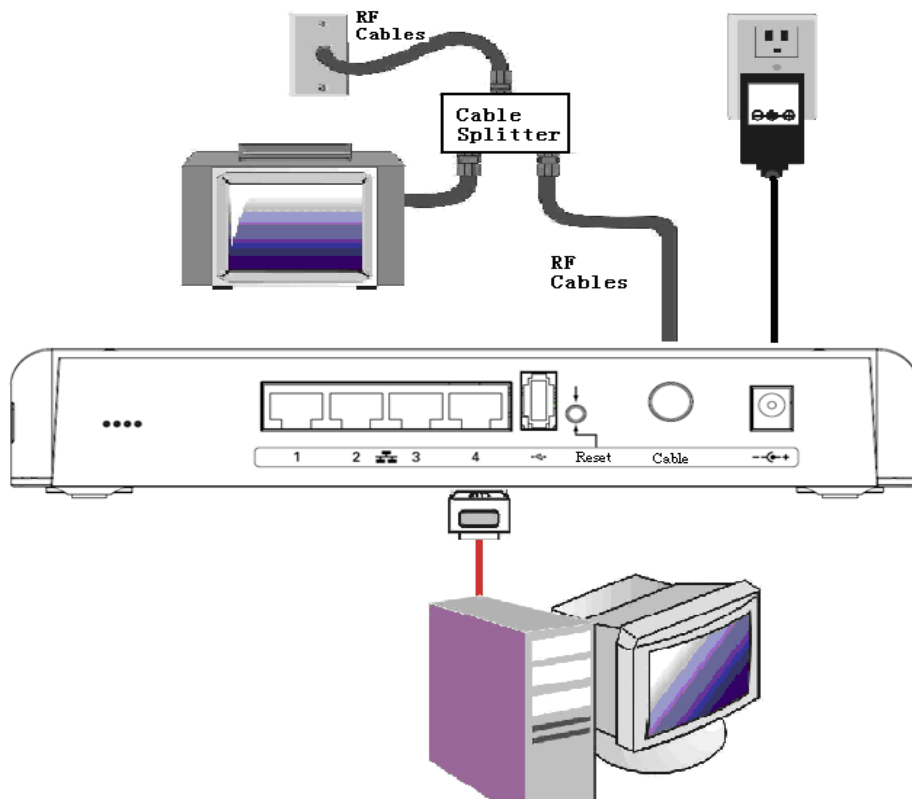
Fig.2: Ethernet Connection
