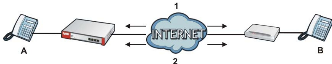
Figure 201 H.323 ALG Example
