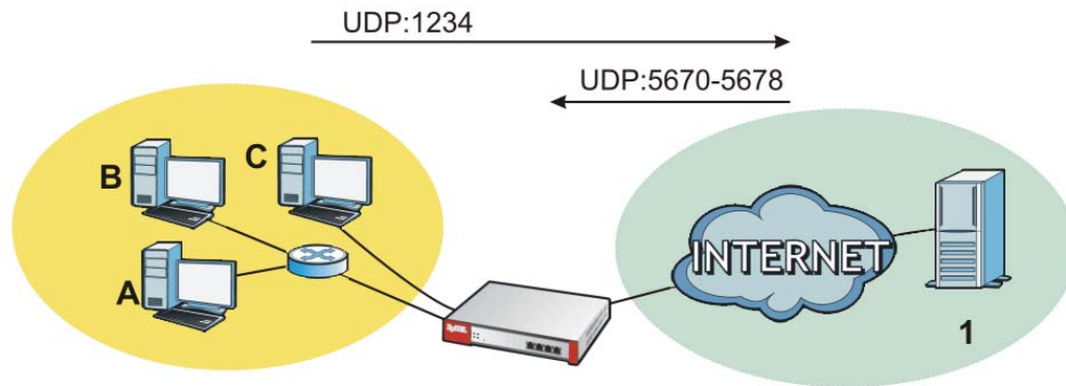
Figure 179 Trigger Port Forwarding Example
