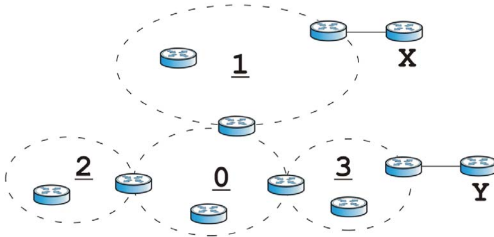
Figure 181 OSPF: Types of Areas
