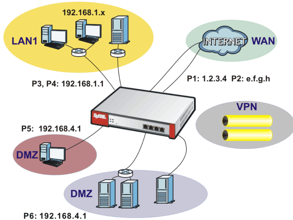
Figure 55 Ethernet Interface, Port Roles, and Zone Configuration Example
