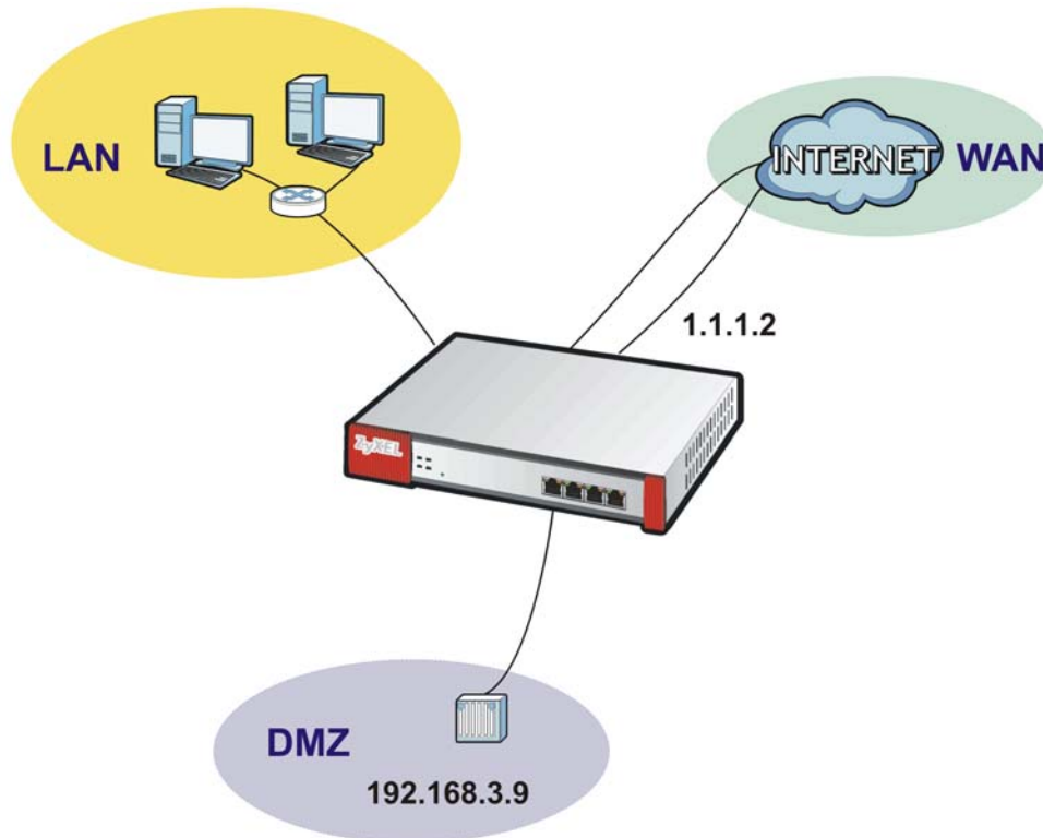
Figure 105 IPPBX Example Network Topology
