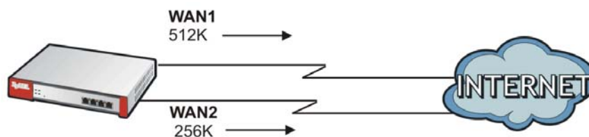
Figure 169 Least Load First Example
