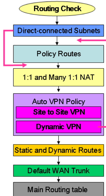
Figure 53 Routing Table Checking Flow
