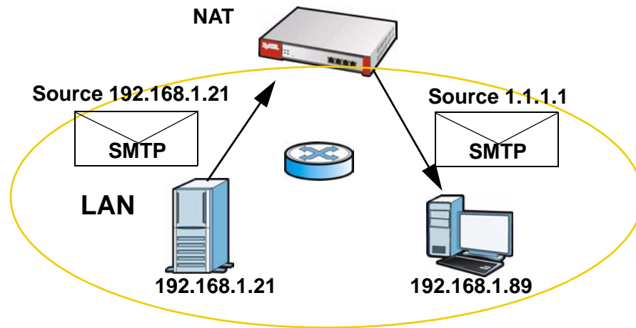
Figure 196 LAN to LAN Return Traffic
