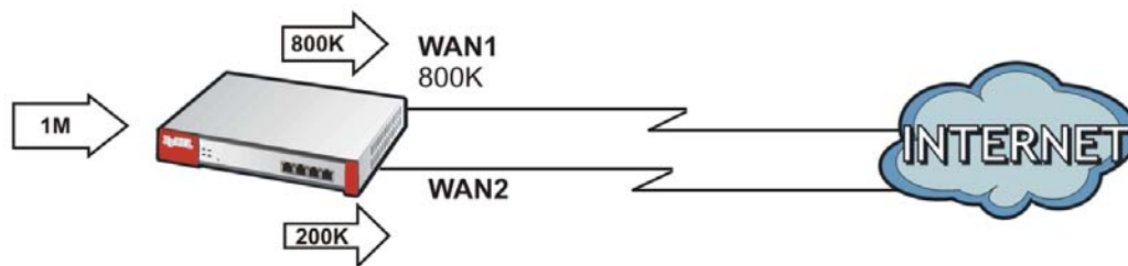
Figure 170 Weighted Round Robin Algorithm Example
