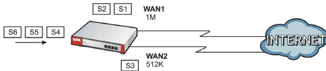
Figure 171 Spillover Algorithm Example
