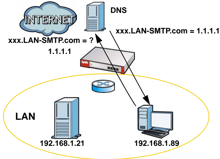
Figure 194 LAN Computer Queries a Public DNS Server
