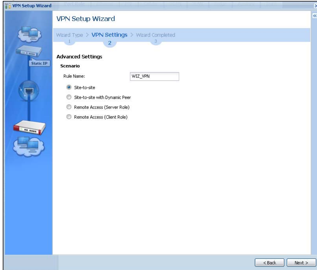
Figure 47 VPN Advanced Wizard: Scenario
