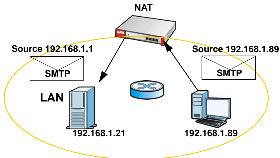
Figure 195 LAN to LAN Traffic
