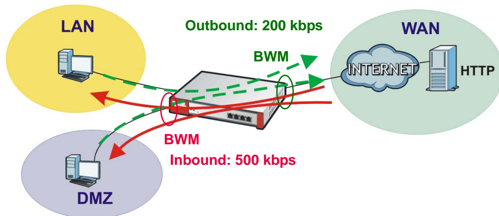
Figure 272 HTTP Any to WAN Bandwidth Management Example
