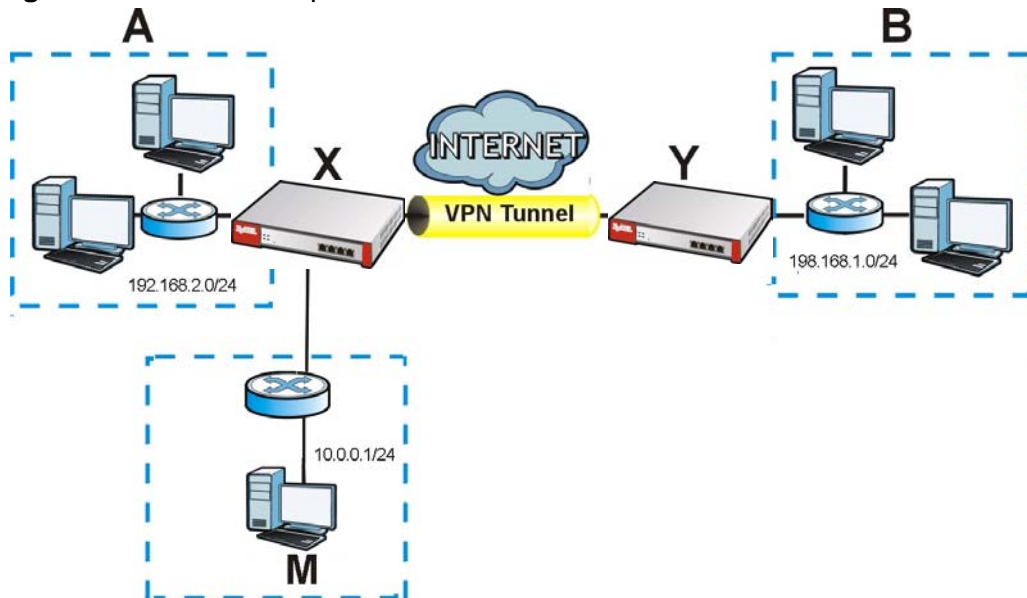
Figure 239 VPN Example: NAT for Inbound and Outbound Traffic
