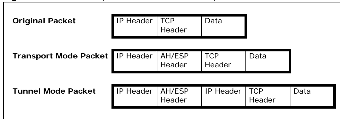
Figure 238 VPN: Transport and Tunnel Mode Encapsulation
