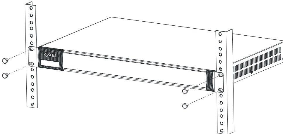
Figure 2 Rack Mounting
