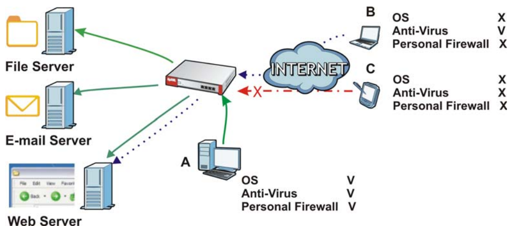
Figure 379 Endpoint Security
