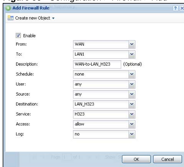
Figure 99 Configuration > Firewall > Add
