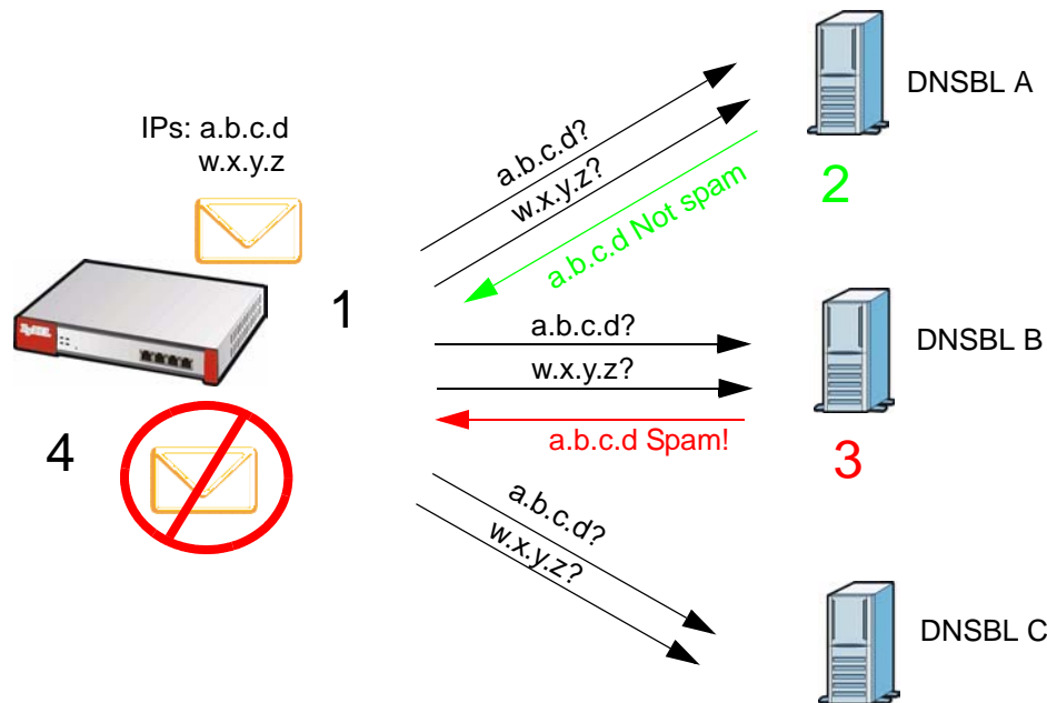
Figure 333 Conflicting DNSBL Replies Example
