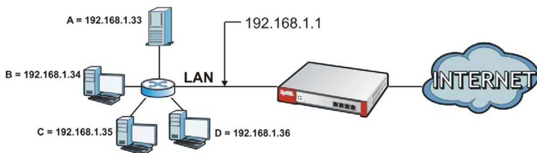
Figure 191 Multiple Servers Behind NAT Example
