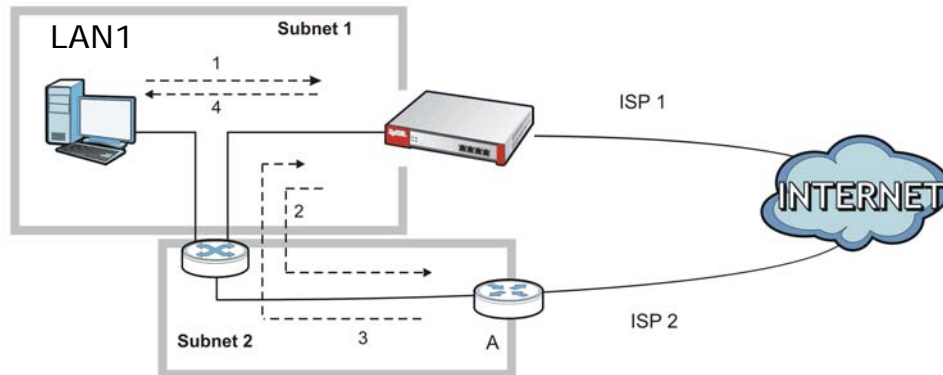
Figure 222 Using Virtual Interfaces to Avoid Asymmetrical Routes
