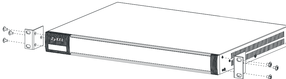
Figure 1 Attaching Mounting Brackets and Screws
