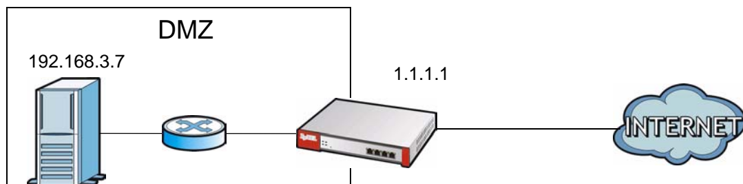
Figure 100 Public Server Example Network Topology
