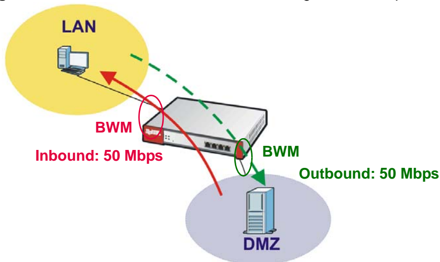
Figure 274 FTP LAN to DMZ Bandwidth Management Example
