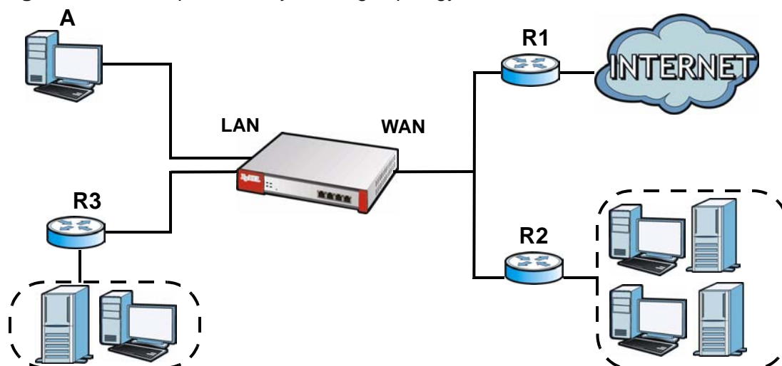
Figure 174 Example of Policy Routing Topology
