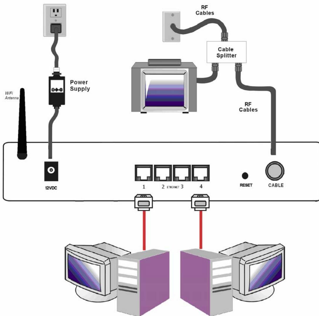
Fig.3: Multiple-PC Connection
