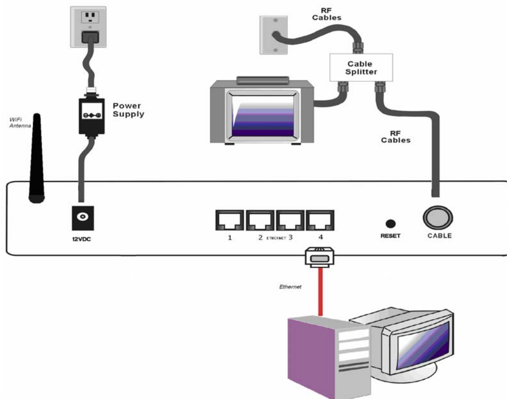
Fig.2: Ethernet Connection
