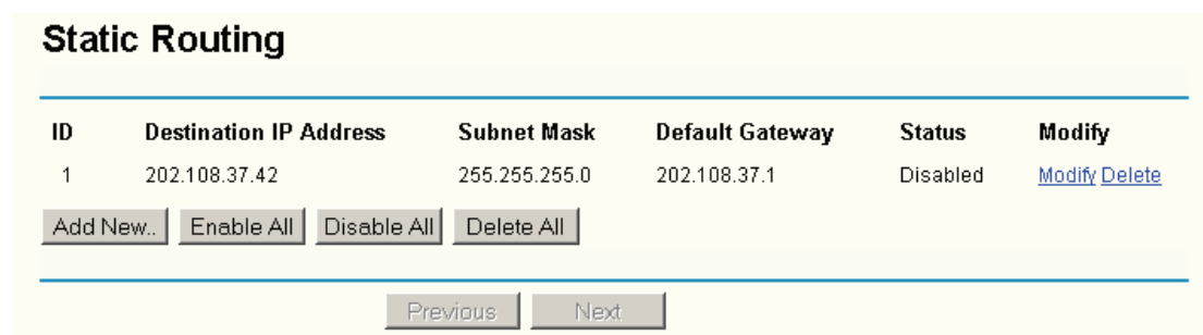
Figure 4-49 Static Routing
