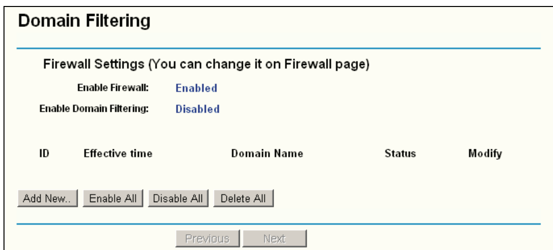
Figure 4-37 Domain Filtering
