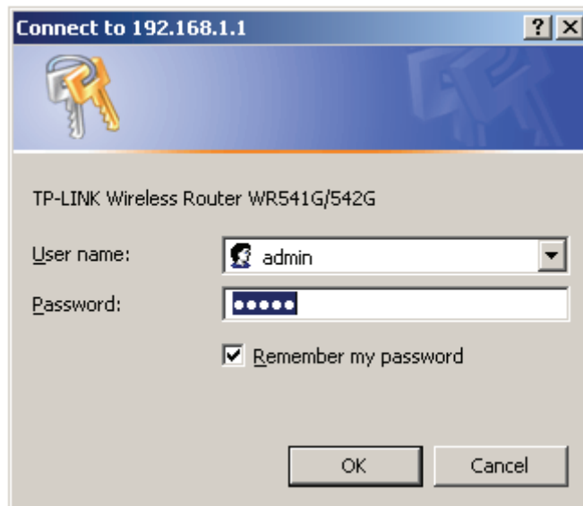
Figure 3-4 Login Windows
