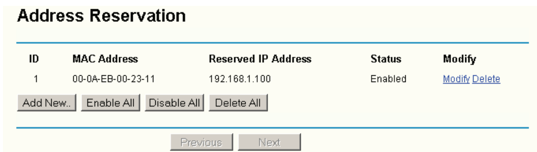
Figure 4-24 Address Reservation
