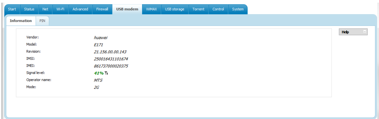
Figure 112. The USB modem / Information page.
